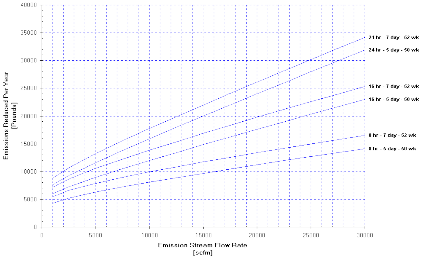
Figure C2-1: Cost Effectiveness Curves for Thermal Oxidation Systems for POC Control Based on cost-effective trigger level of $17,500/ton POC reduced
